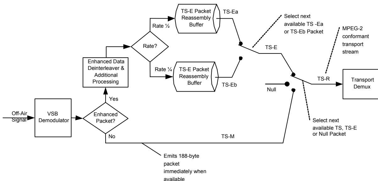
Figure C3 Reference receiver model.
