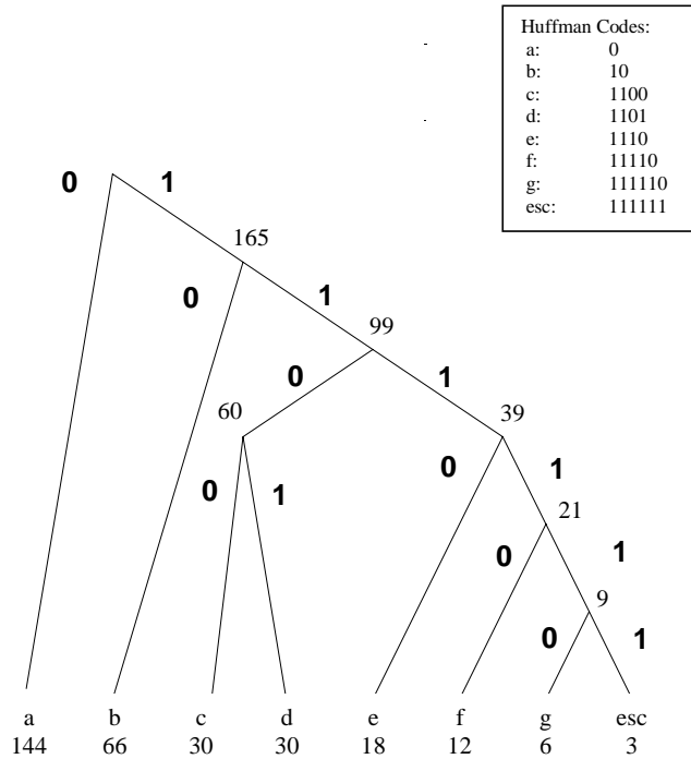
Figure F1 Example Huffman tree.
